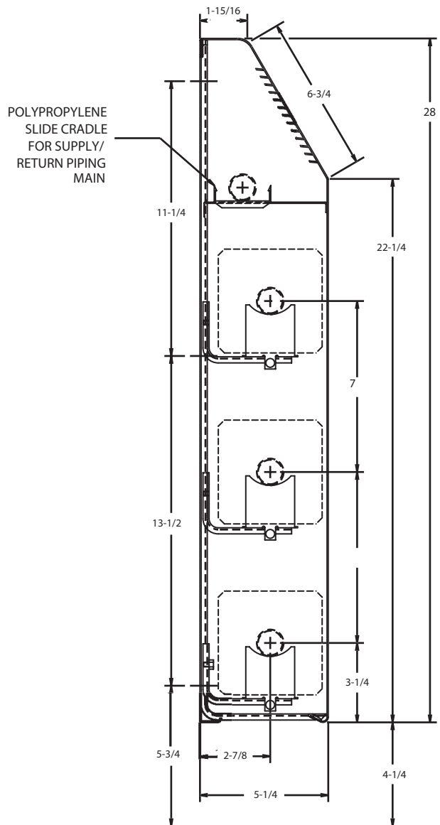
"JA-28" SERIES ENCLOSURES WITH FULL BACK PANEL AND SLIDE CRADLE FOR SUPPLY/RETURN PIPING
