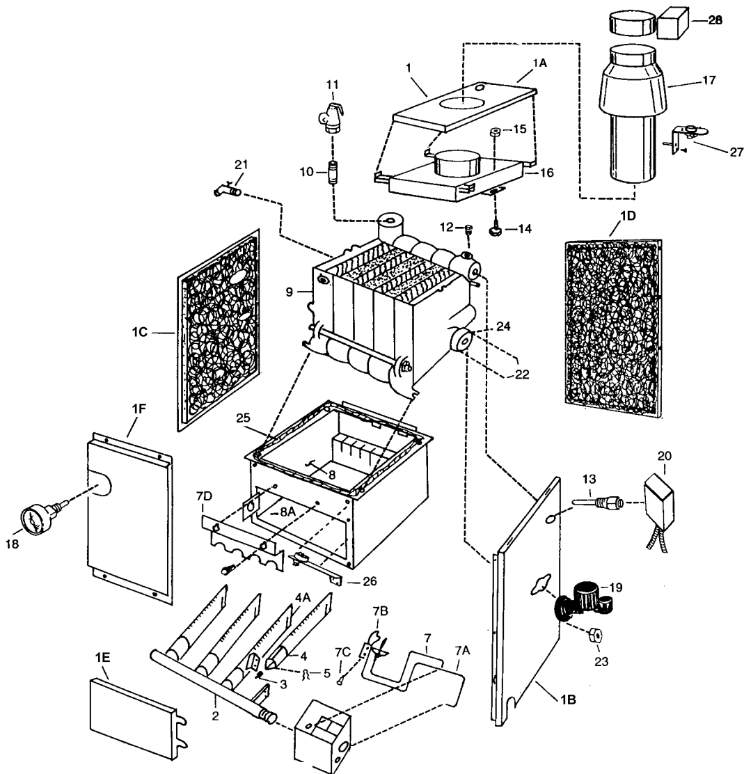
Ignition Control (mounts on jacket)
