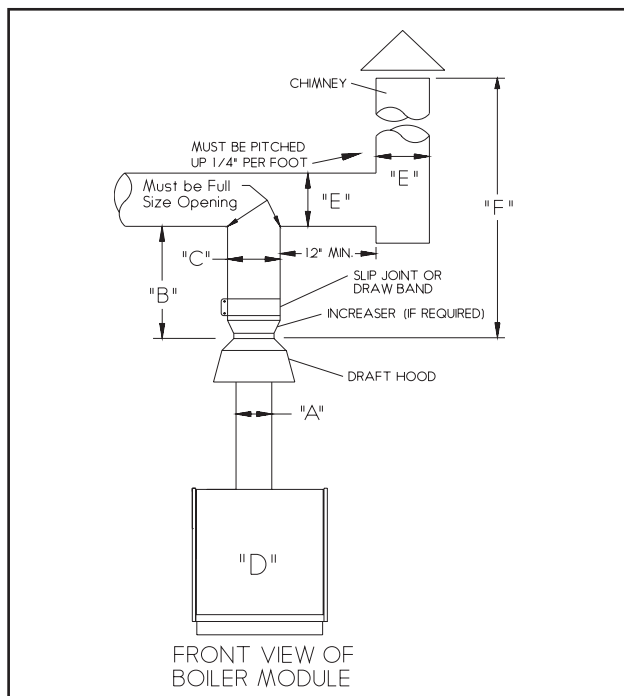
Figure 9. Connector rise
